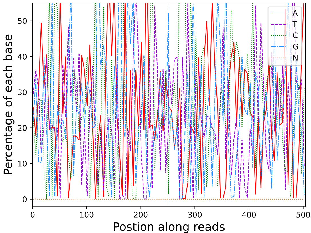
Base percentage along reads (R10325)
